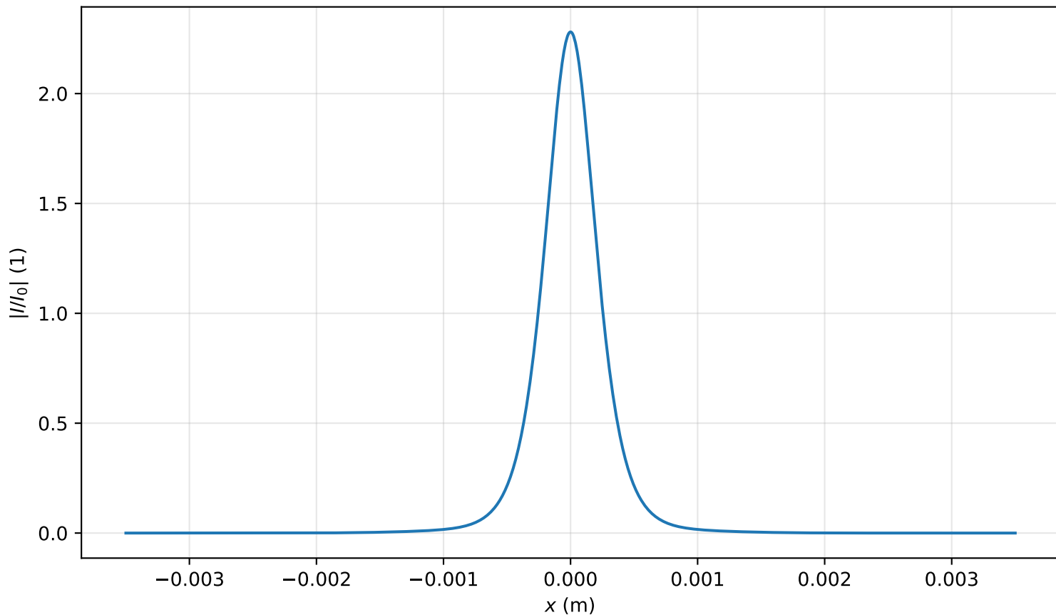
Intensity profile I(x, y = 0, z = 2.309m)/I_0 , P_{in}=1.0P_{cr} , artificial time
